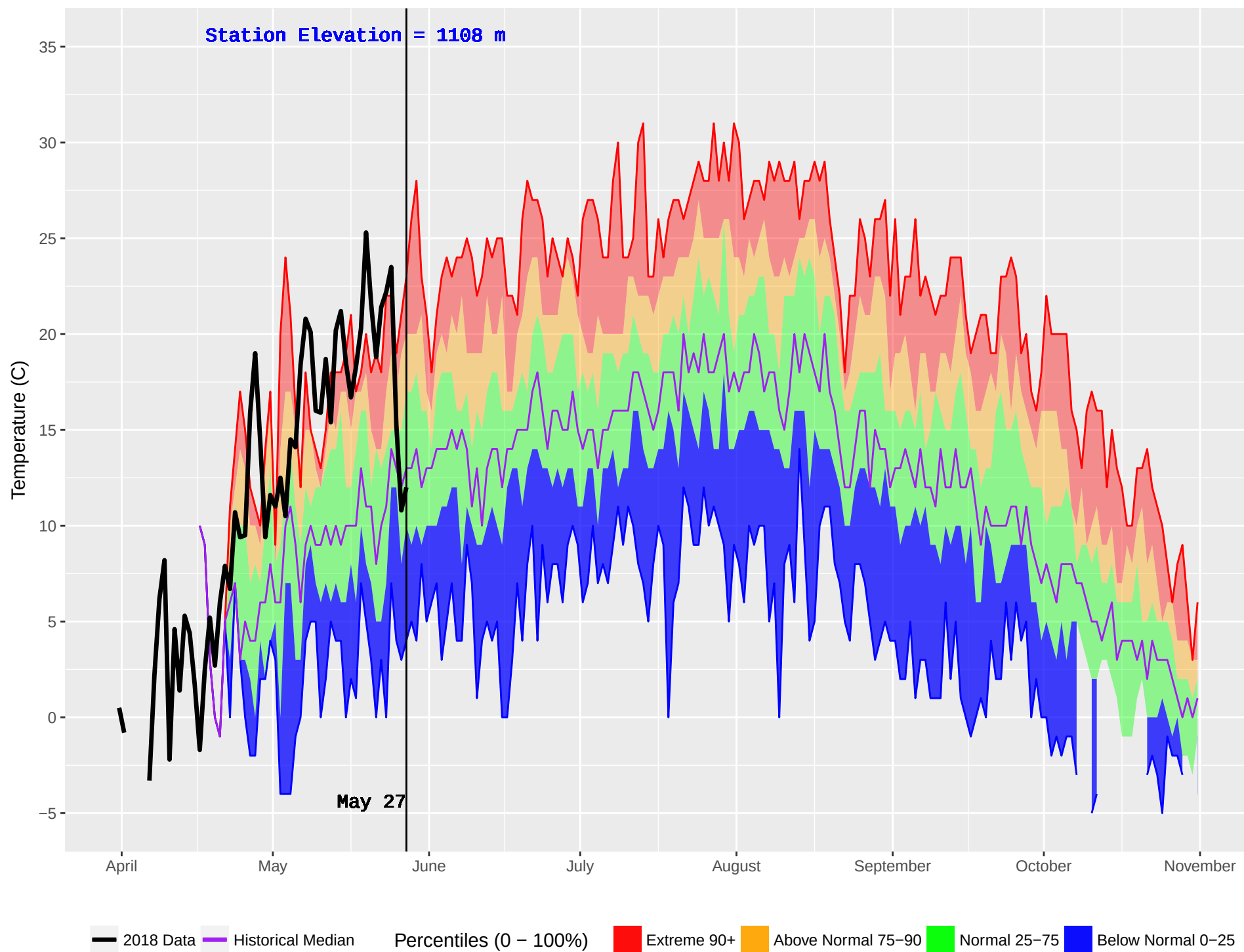
NABESHE (151) : Historical (1987–2016) and Current (2018) Noon Temperature
